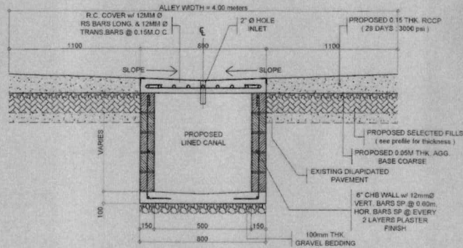
SECTION DETAIL OF LINE CANAL
