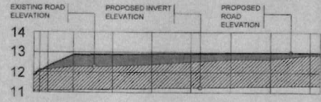
ROAD PROFILE
