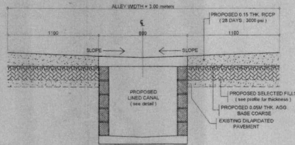
ROAD CROSS SECTION
