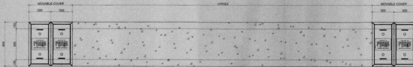
PLAN OF .80M CHB LINED CANAL
