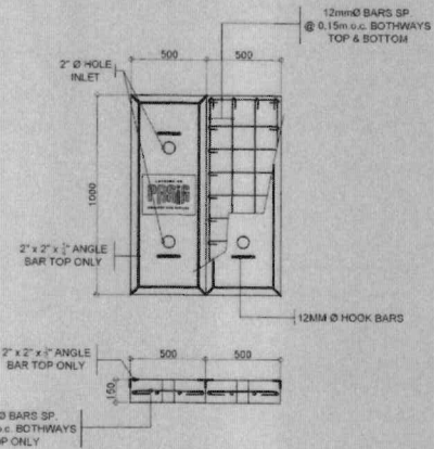
MANHOLE COVER DETAIL
